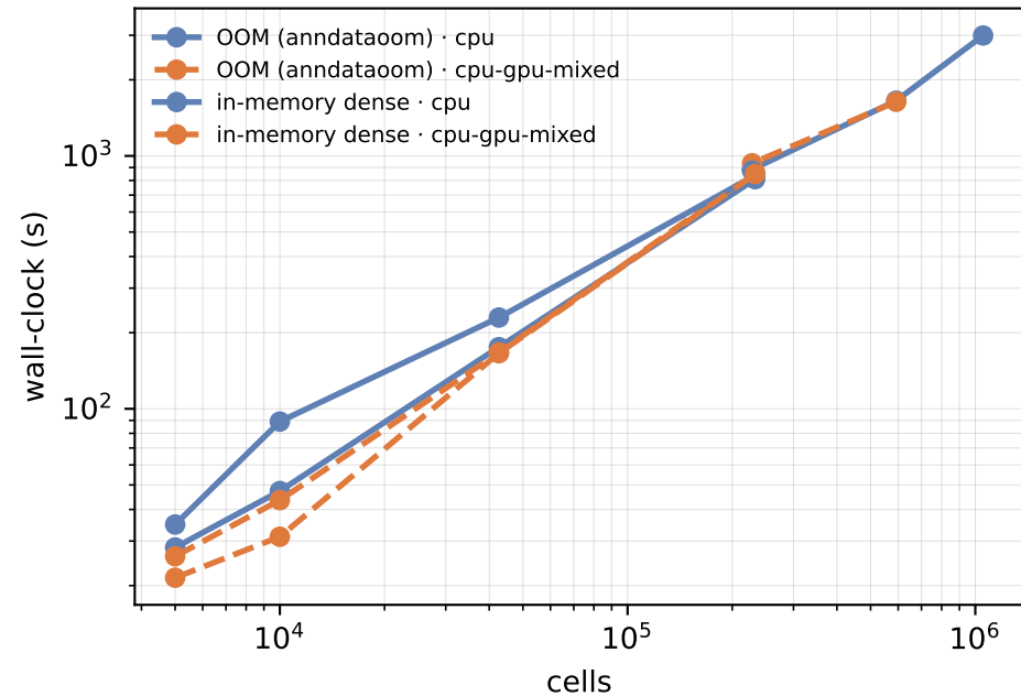
(a) cpu vs cpu-gpu-mixed: pipeline time
