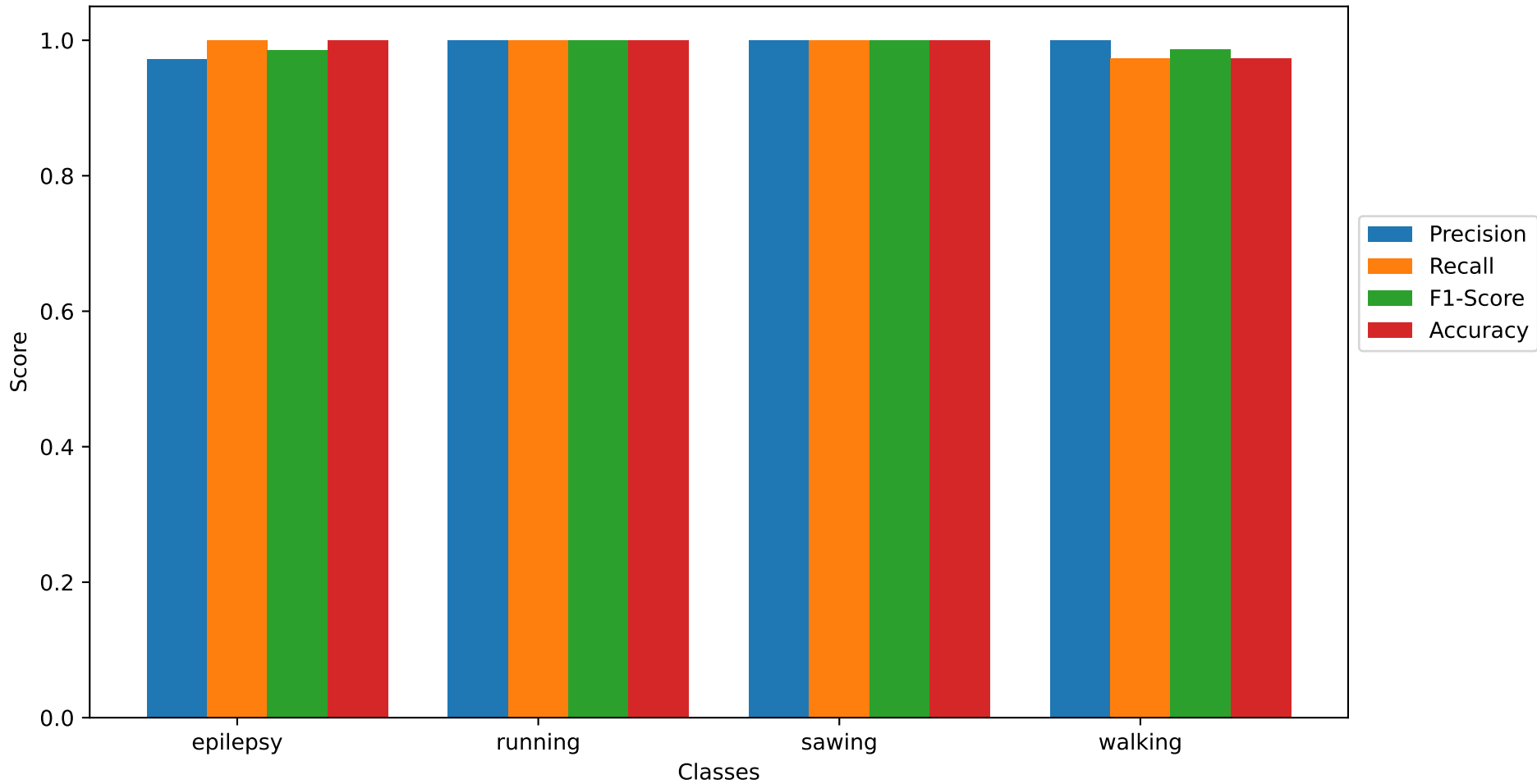
Per-Class Metrics Overall Accuracy: 99.28%, Cohen's Kappa: 0.99, MCC: 0.99
