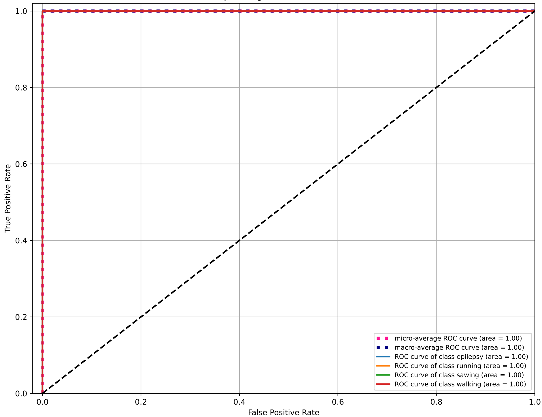
Receiver Operating Characteristic for Multiclass
