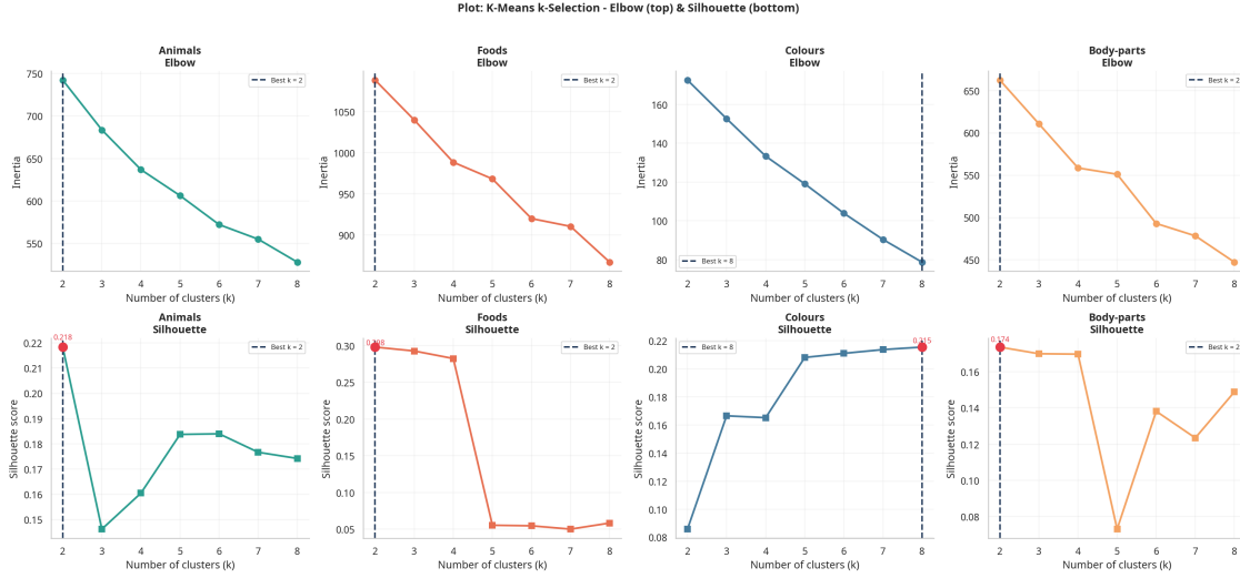
Figure 9: K-Means k -Selection: Elbow (top) and Silhouette (bottom) by Domain. Red dot marks optimal k . Animals, foods, body-parts converge on k=2 (silhouettes: 0.218, 0.298, 0.174). Colours requires k=8 (silhouette=0.215), reflecting fine-grained chromatic distinctions in its 27-word vocabulary. Elbow plots confirm diminishing inertia returns beyond optimal k .
