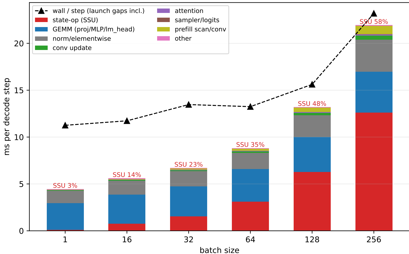
Decode-step latency breakdown vs batch (B200, eager, fp32 state)
