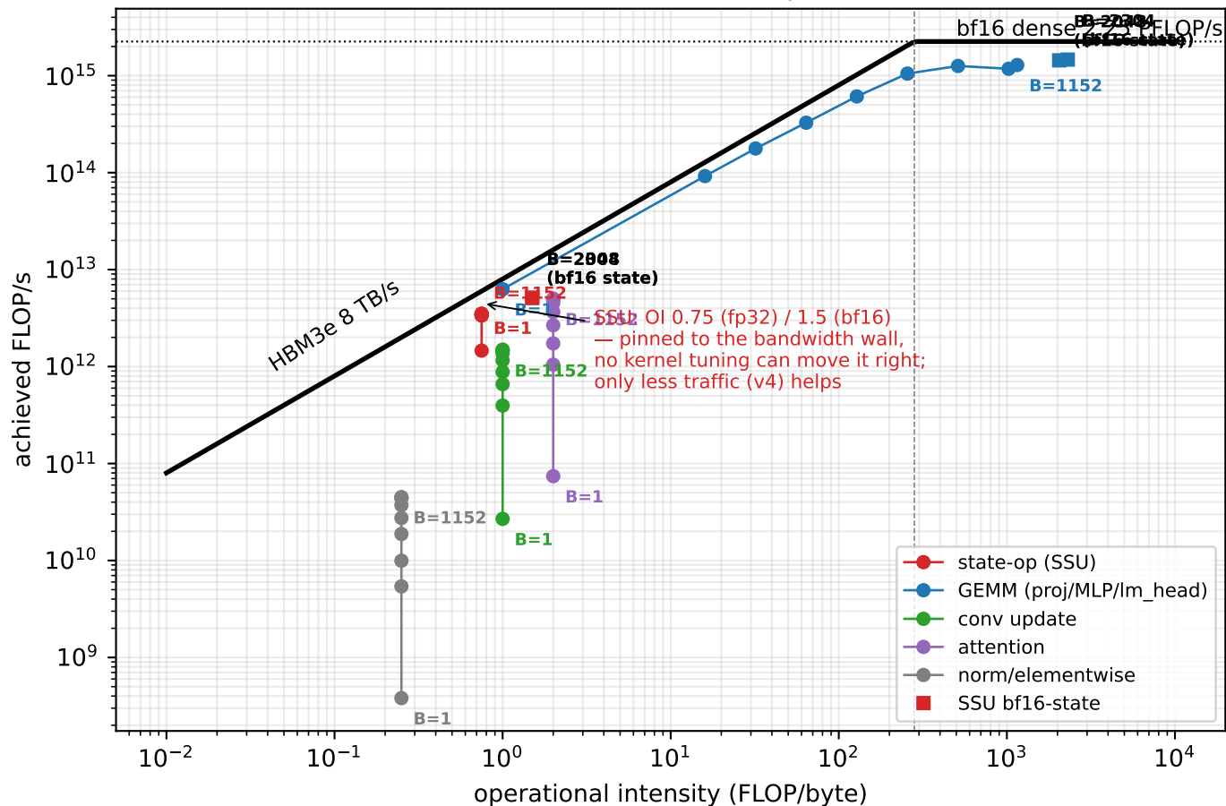
B200 roofline — Nemotron-9B decode components (vLLM, measured)
