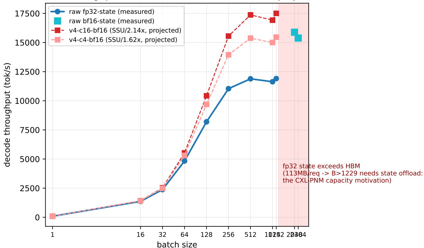
Decode throughput vs batch — raw measured + v4 projection
