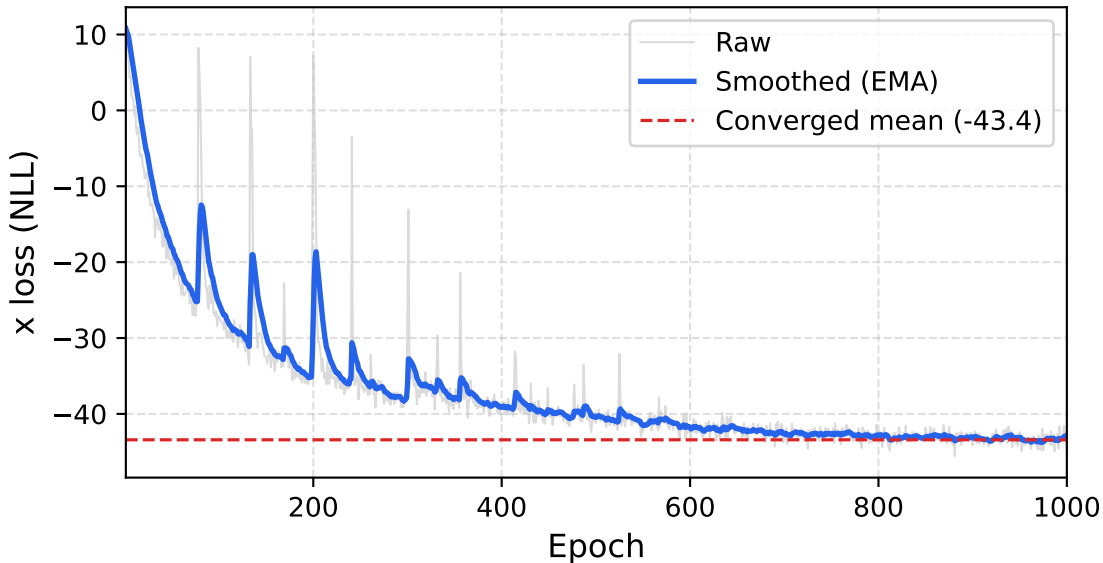
RIBBO on BBOB Rastrigin — Training Convergence
