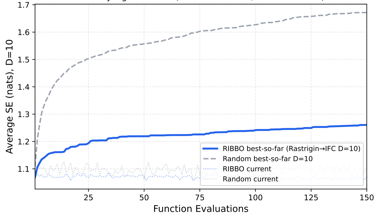
Zero-shot Transfer: Rastrigin D=10 \rightarrow IFC SE D=10 200 Rayleigh channels (solid=best-so-far, dotted=current)
