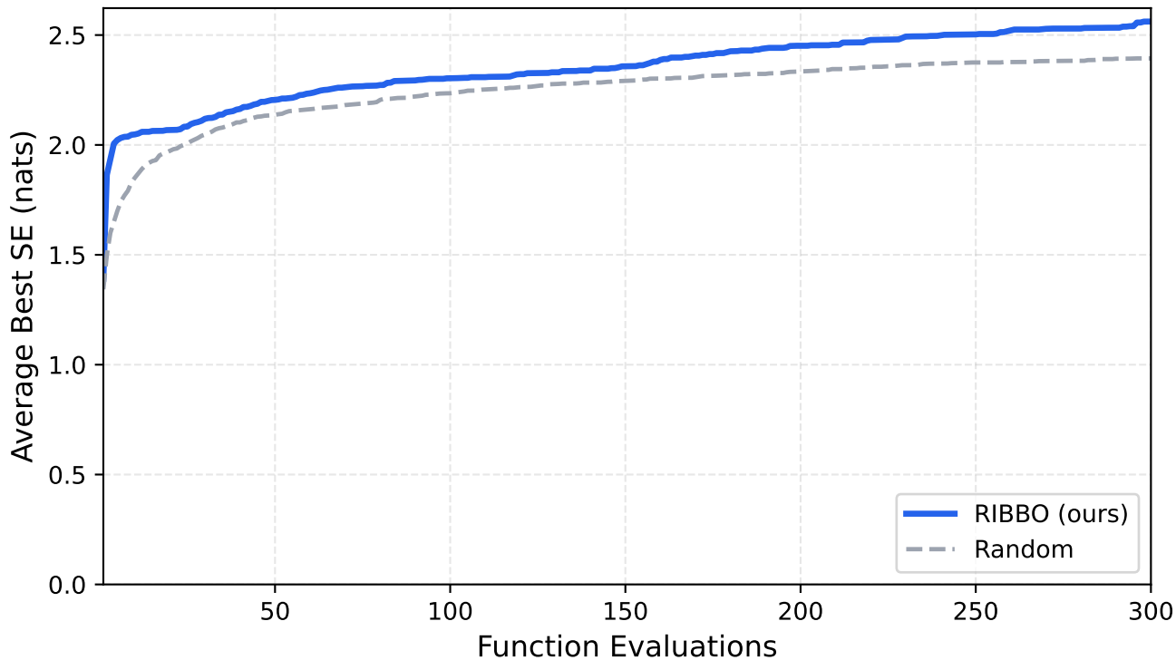
Convergence Behavior — IFC SE ( D=3 , P_{tx}=10 W) 200 Rayleigh fading channels, avg over channels
