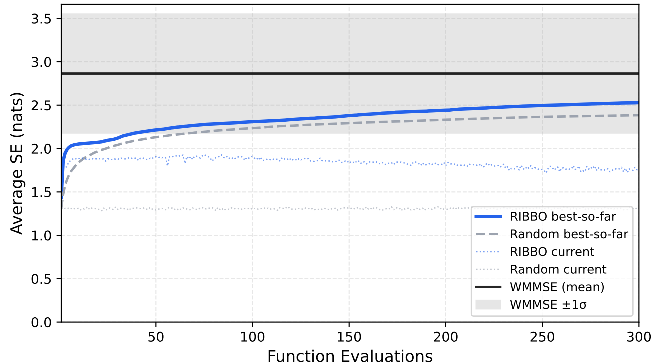
Convergence Behavior — IFC SE ( D=3 , P_{tx}=10 W) 500 channels \times 3 ep (solid=best-so-far, dotted=current, black=WMMSE)
