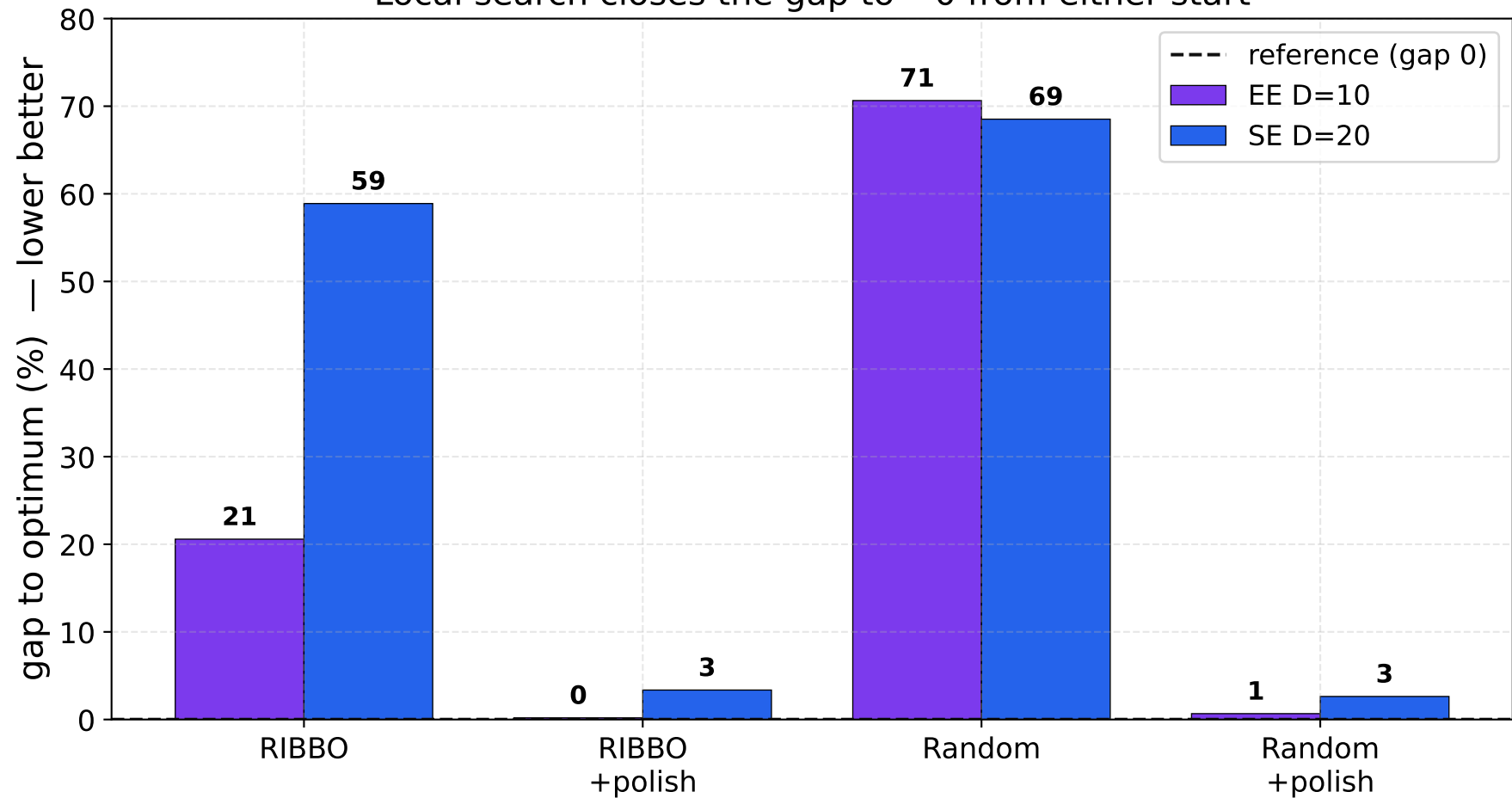
Local search closes the gap to ~0 from either start
