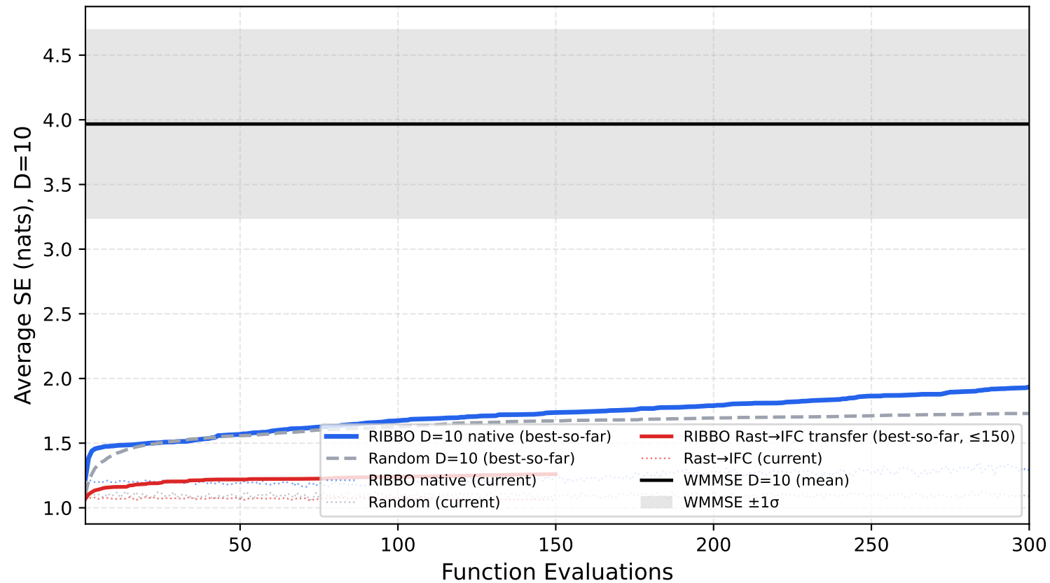
IFC SE D=10 — Native training vs Rastrigin transfer vs WMMSE 200 unseen Rayleigh channels
