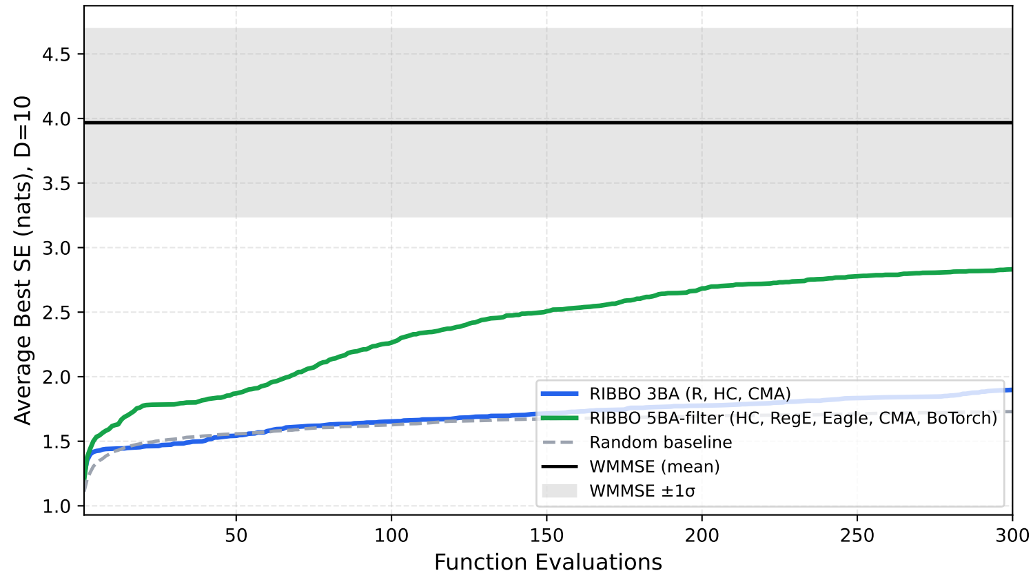
BA-pool ablation — IFC SE D=10 (3BA / 5BA-filter) 200 unseen channels \times 1 ep \times 300 steps
