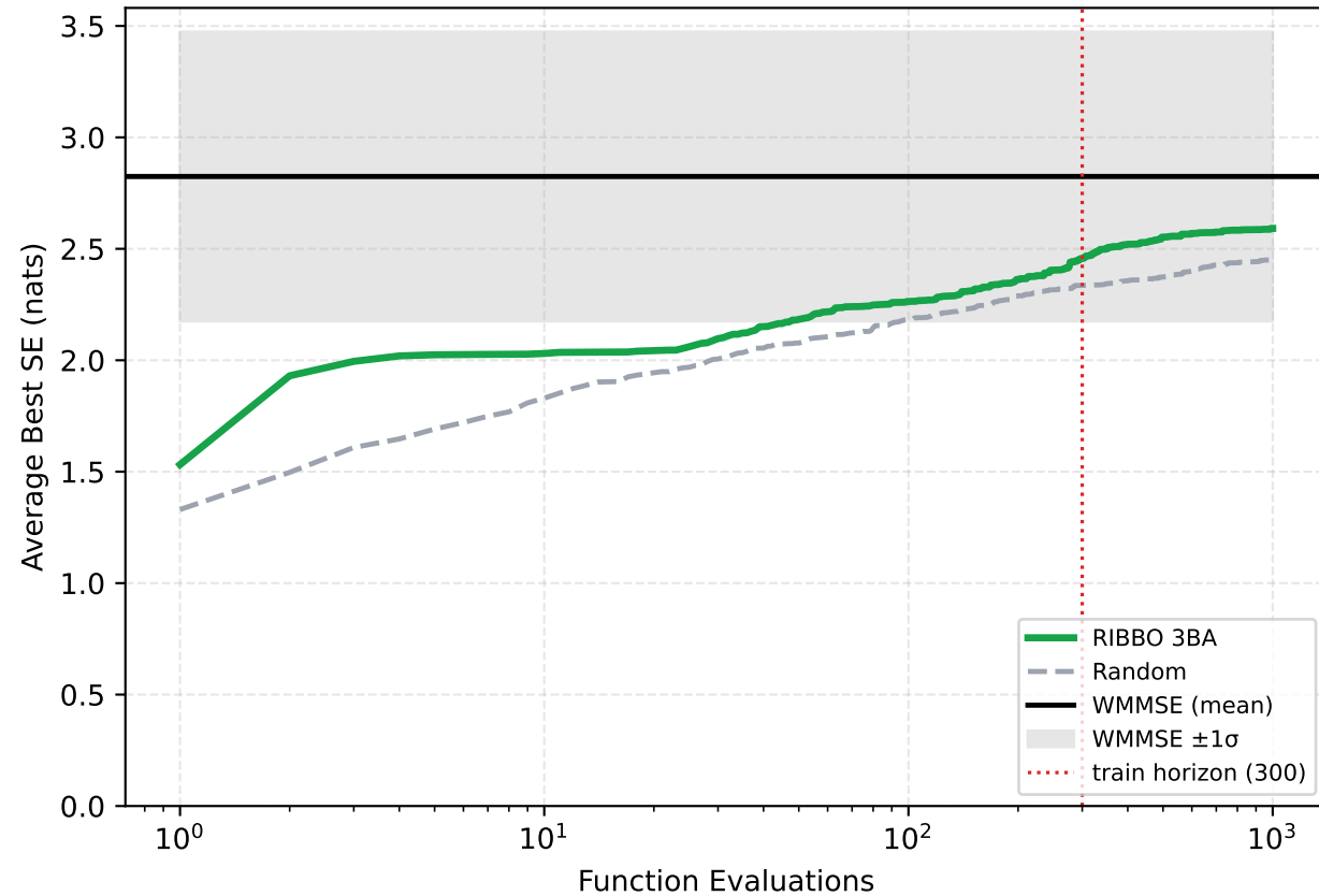
IFC SE D=3 — evaluation budget extended to 1000 final RIBBO = 91.7% of WMMSE (@300: 87.0%)
