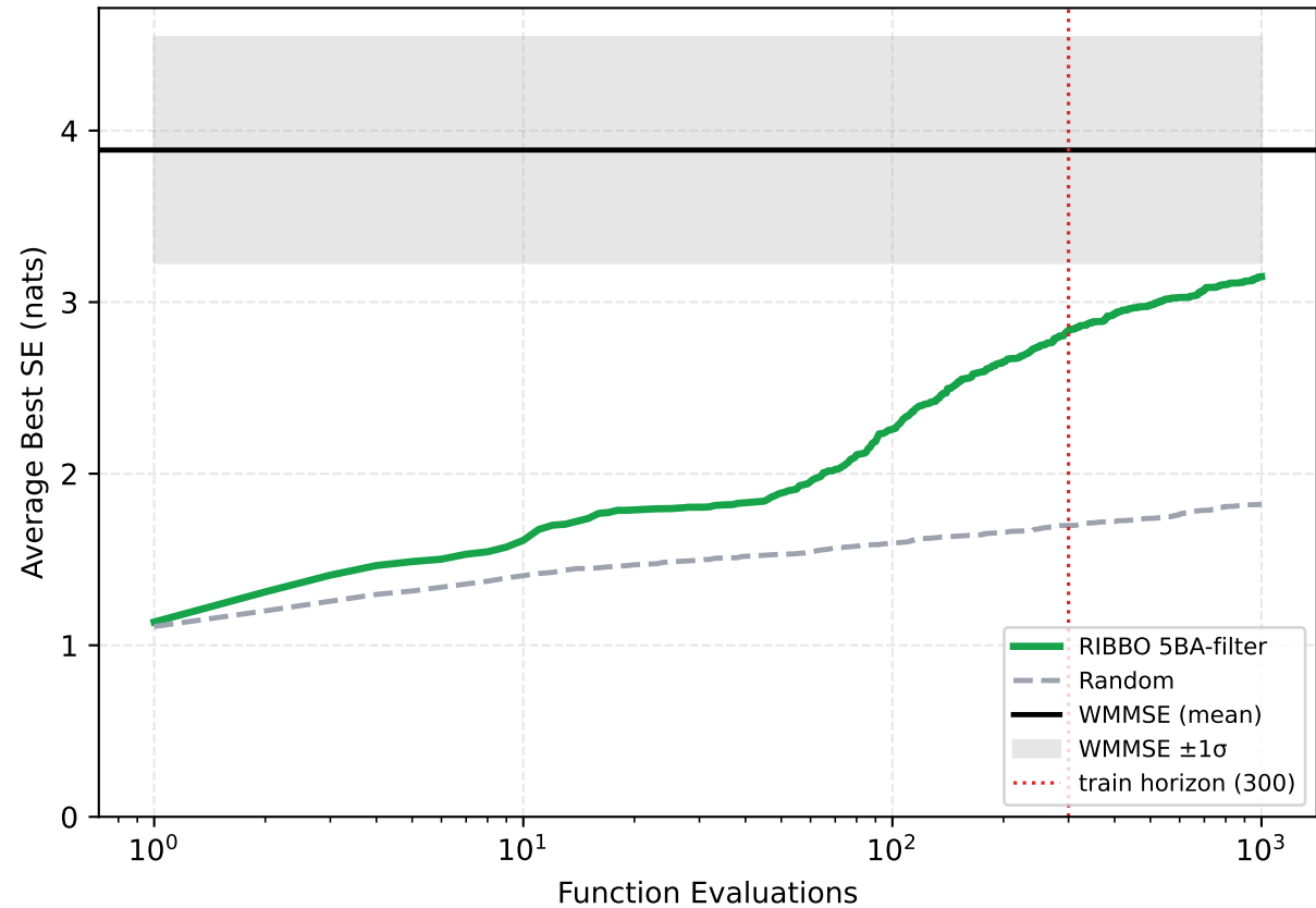
IFC SE D=10 — evaluation budget extended to 1000 final RIBBO = 81.0% of WMMSE (@300: 72.9%)
