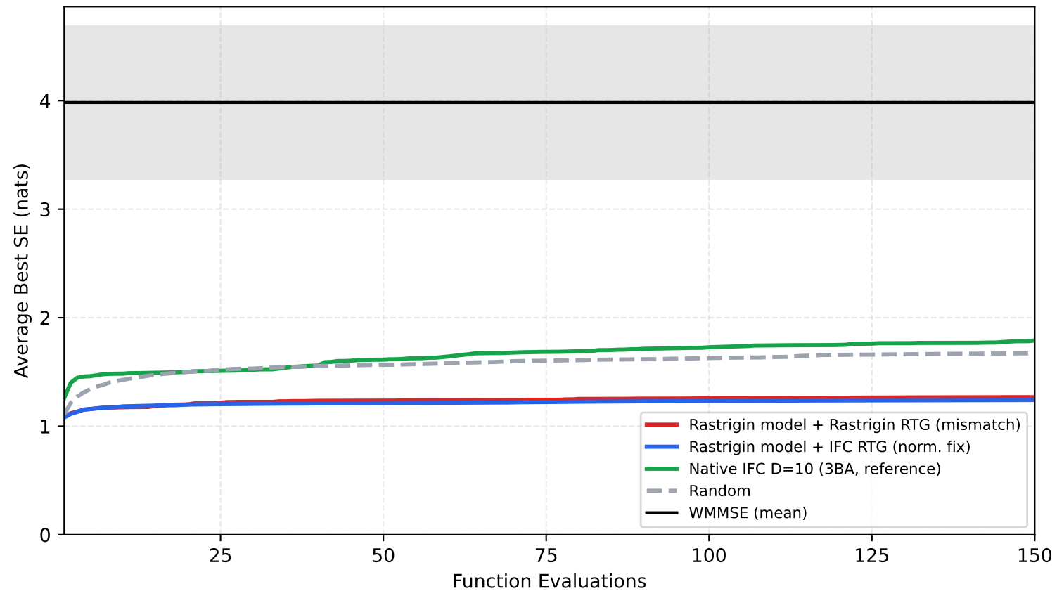
Rastrigin->IFC D=10 transfer: does fixing RTG normalization help? 150 unseen channels \times 150 steps
