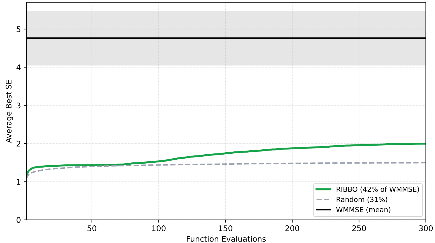
IFC SE D=20 4BA-filter 200 unseen channels \times 300 steps
