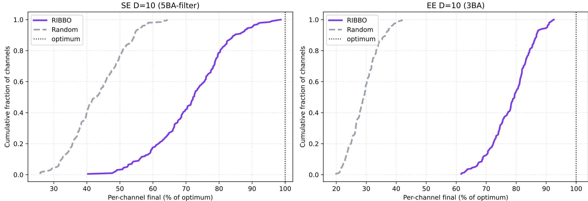
Per-channel CDF: RIBBO distribution is shifted toward the optimum
