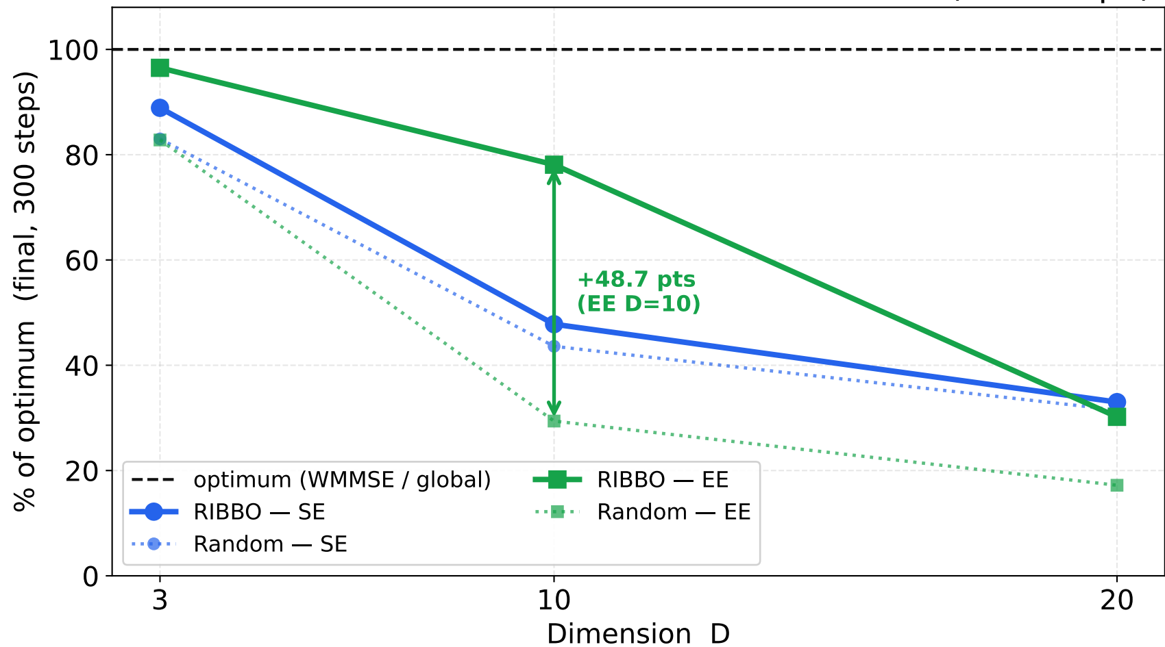
RIBBO vs Random across dimension — SE and EE (3BA recipe)
