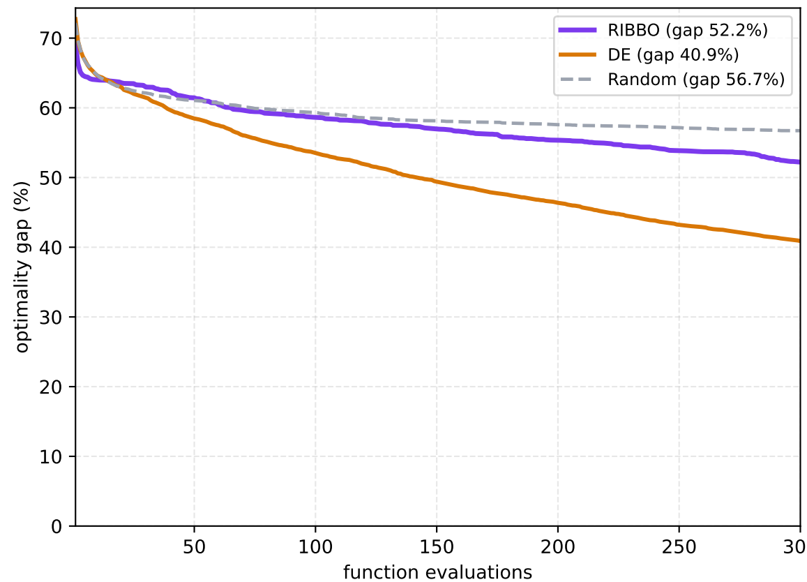
IFC SE D=10 (3BA) (200 unseen channels)
