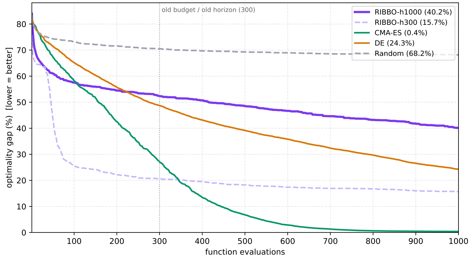
IFC EE D=10 (100 ch) — RIBBO retrained at horizon 1000 (fair) vs CMA-ES@1000
