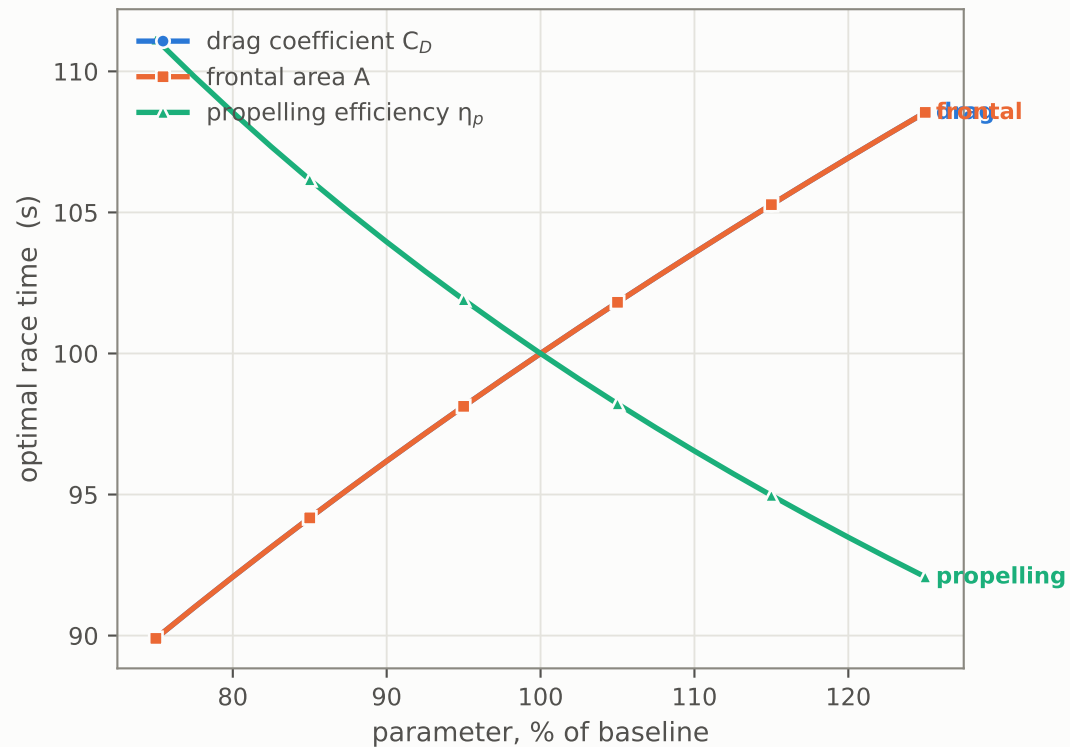
Drag sets the race time
