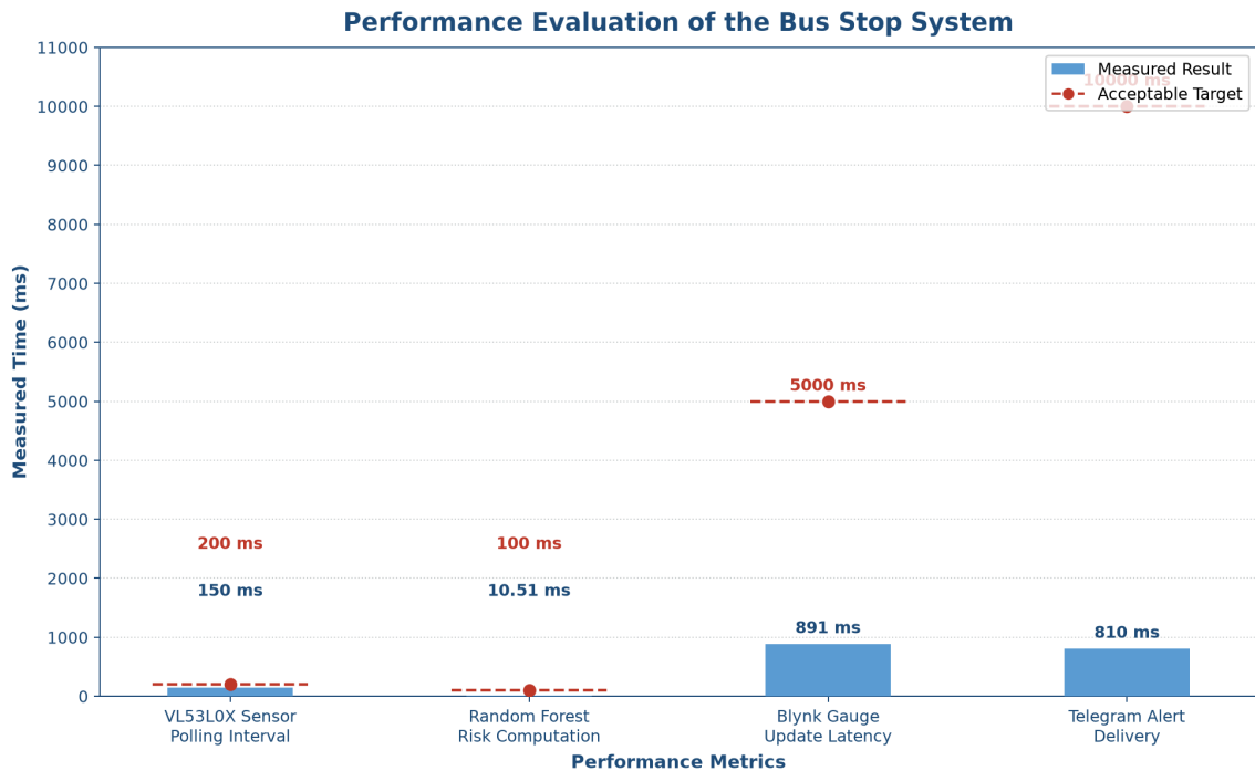
Figure 5.6: Performance comparison of measured system response times against acceptable target limits.
