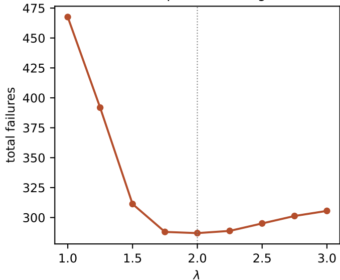
Indicator-coupled variant: artifactual interior optimum (fine grid)
