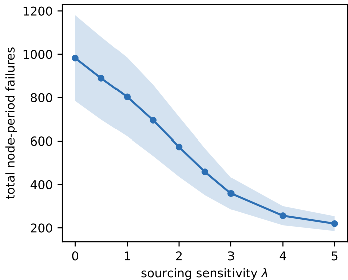
Corrected model: monotone benefit (95% CI)
