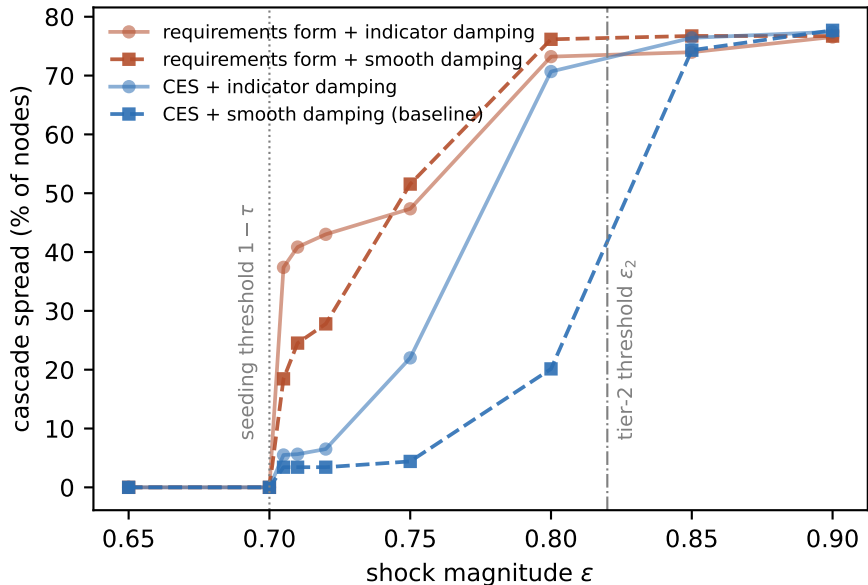
Spread versus shock depth, four coupling specifications
