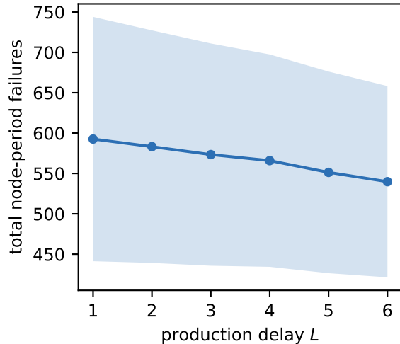
T = 50 (censored 19-25%)
