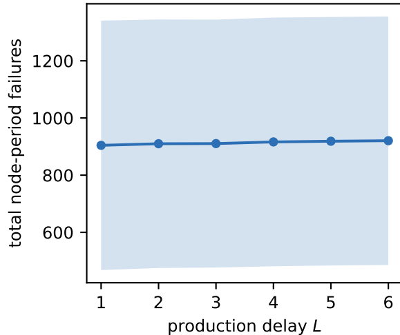
T = 200 (uncensored)
