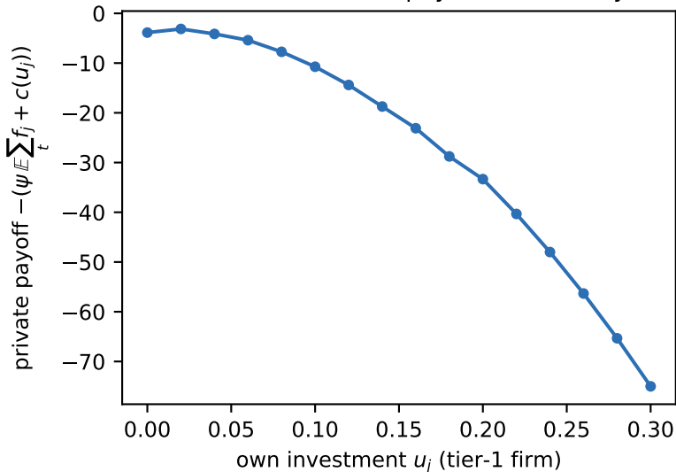
Numerical check of payoff unimodality
