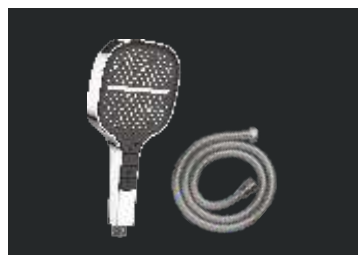
28190 ABS Hand Shower 3 Function With 1.5 mtr Flexible Hose Size : 130 x 130 mm | MRP : ₹ 4,500/- Flows : Shower, Mist, Waterfall Shower
