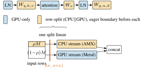
Figure 2. FusionML per-layer prefill split. Every linear layer is row-split across concurrent CPU/GPU streams behind an eager boundary; attention, normalization, and element-wise math stay on the GPU. The CPU share \rho is calibrated per matmul shape under contention ( \rho \approx 0.25\text{--}0.40 across chips).
