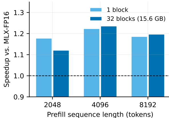
Figure 3: Single block vs. 32 stacked blocks (15.6 GB FP16 weights), M4 24 GB. Depth does not erode the win.
