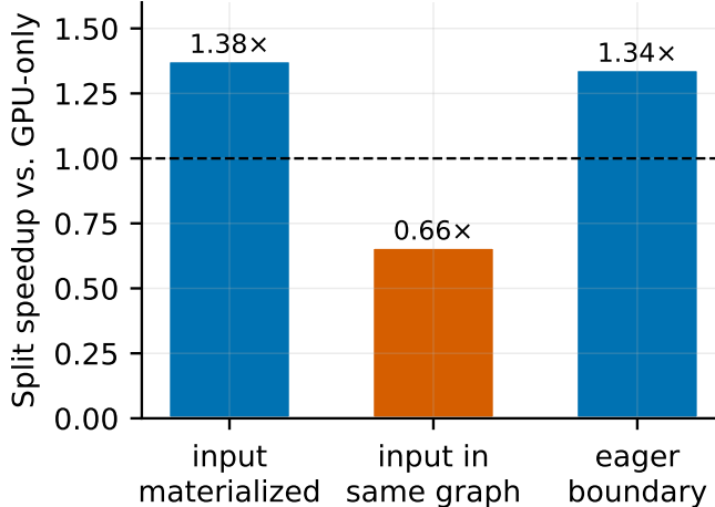
Figure 1: The mechanism probe ( 2048 \times 1600 \times 1600 \times 6400 FP16 matmul, 35% of rows on the CPU stream, M1). The identical split wins 1.38\times when its input is materialized, loses 0.66\times when the input is an unmaterialized GPU result inside the same lazy graph, and wins again ( 1.34\times ) when an eager mx.eval boundary materializes the input first.
