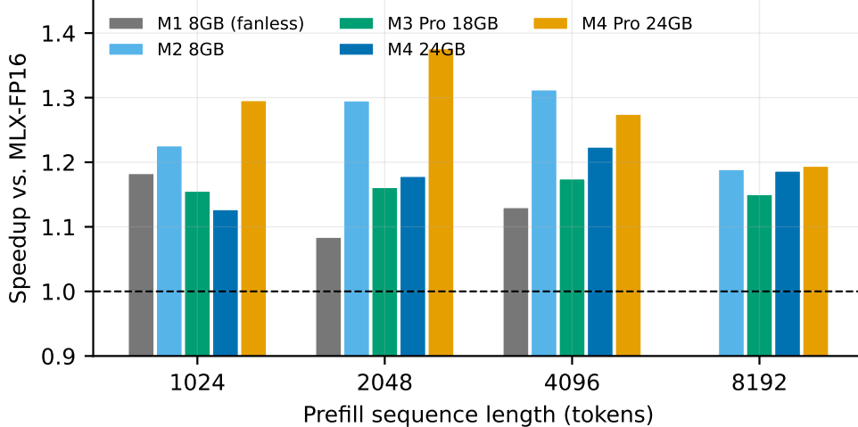
Figure 2: Llama-3-8B-geometry decoder-block prefill: per-layer split speedup over precision-matched MLX-FP16, five chips, seq. 1024–8192. Every actively-cooled chip wins at every length; the fanless 8 GB M1 fades at 8192 under memory pressure and thermal throttling.
