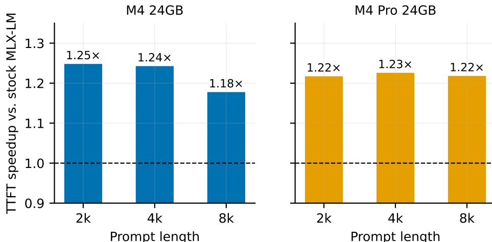
Figure 4: Time-to-first-token speedup for Qwen2.5-7B-Instruct (bf16) served through stock MLX-LM with FusionML’s split patched into nn.Linear (prefill-scale calls only; untuned fixed \rho=0.30 ). Greedy decoding; decode throughput unchanged (7.1→7.1 tok/s on M4, 13.4→13.5 on M4 Pro).
