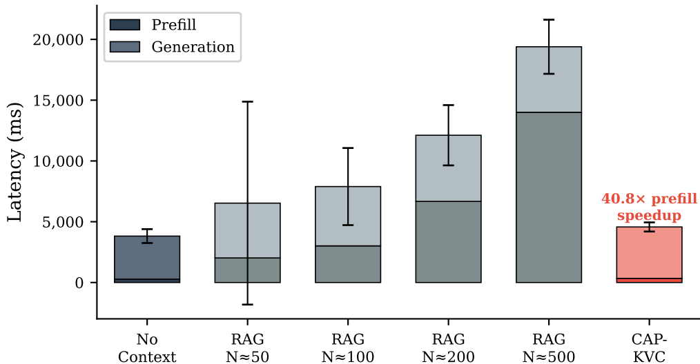
Latency Breakdown: Prefill vs Generation
