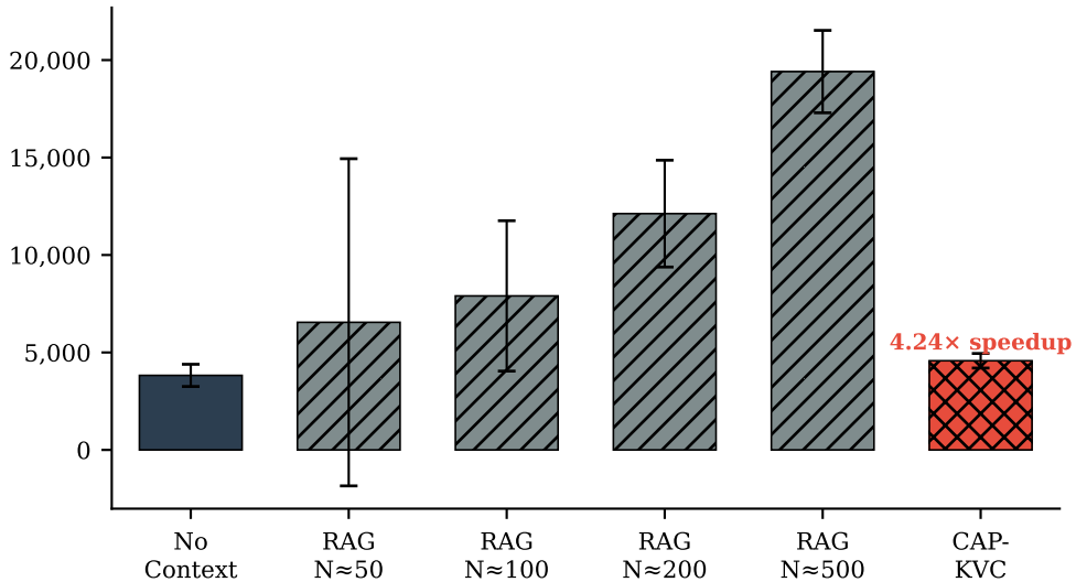
Inference Latency Across Pipeline Conditions
