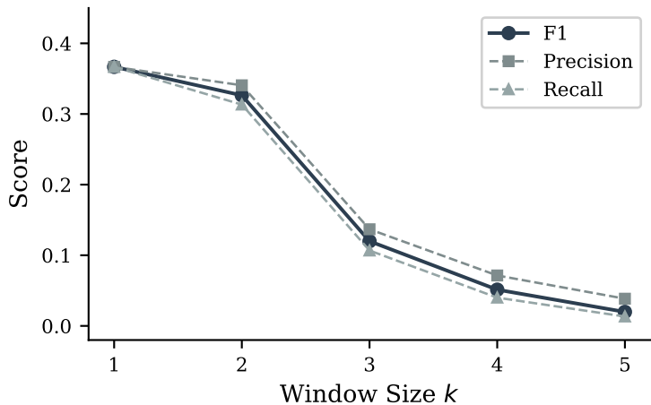
Drift Detection: k-Ablation on DailyDialog
