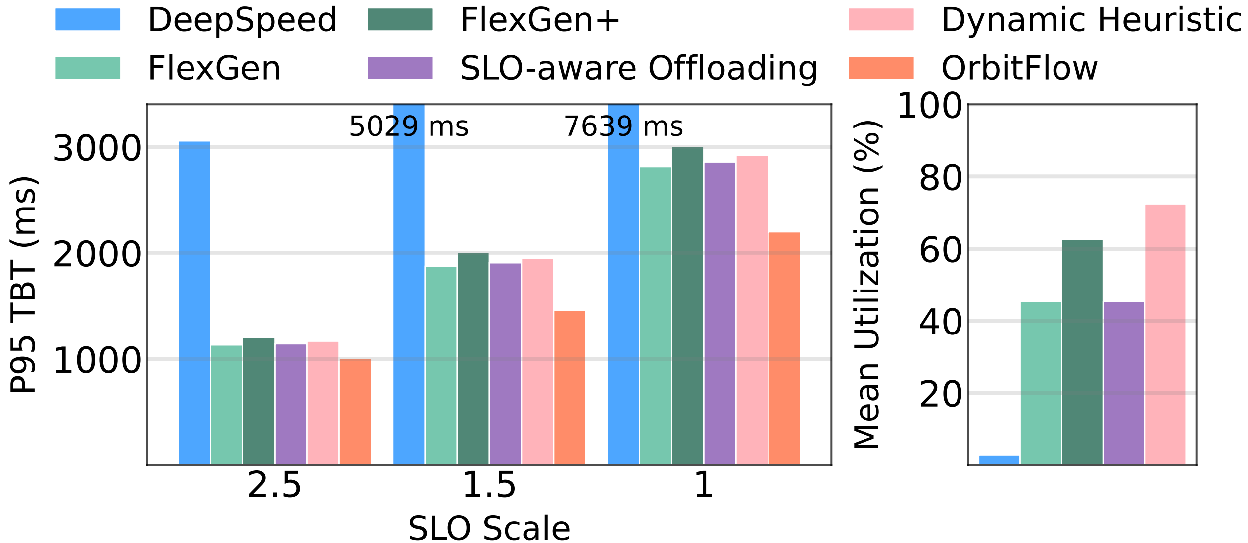
(a) P95 TBT SLO Attainment
