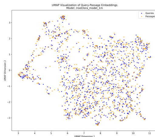
(d) LoRA FT (Random): Reduced semantic differentiation with compressed clustering
