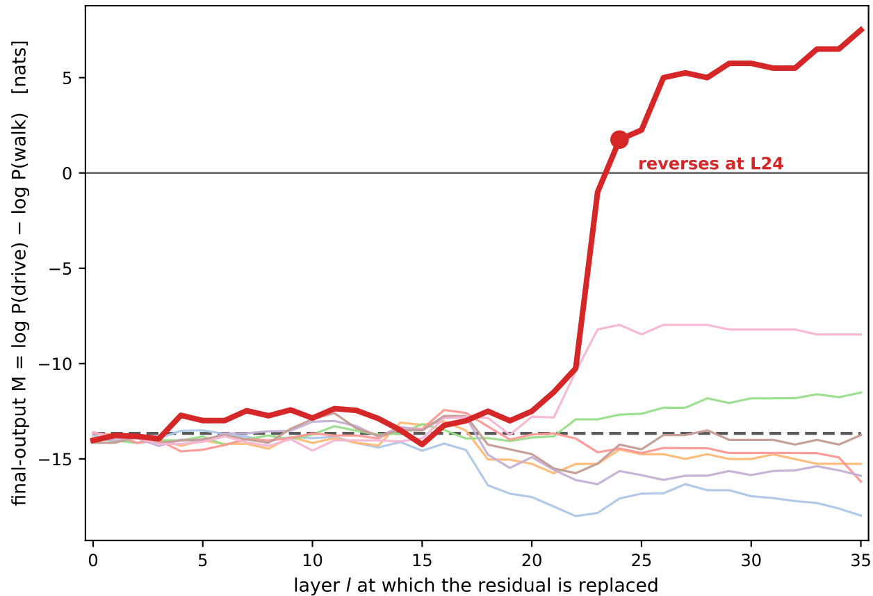
Qwen3-8B: baseline prompt, donor residual patched at layer l
