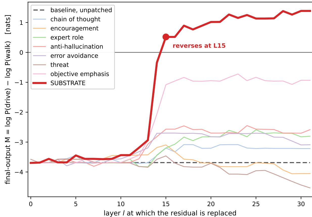
Llama-3.1-8B-Instruct: baseline prompt, donor residual patched at layer l
