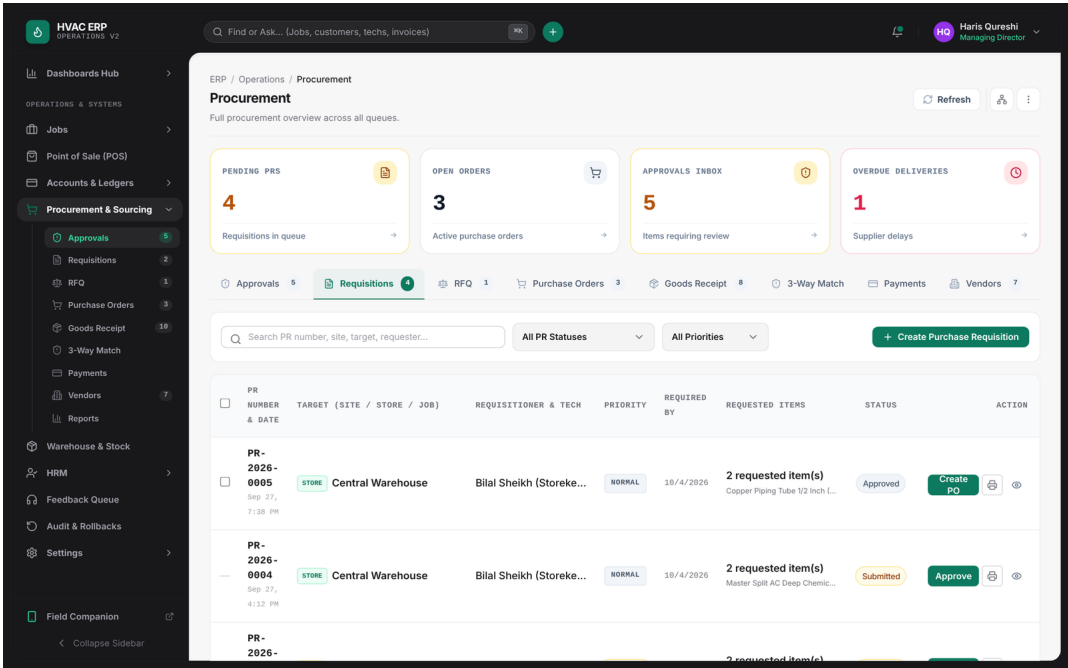
Figure. Procurement hub — Pending PRs, Open Orders, Approvals Inbox, Overdue Deliveries. Requisitions list with Approve / Create PO actions.
