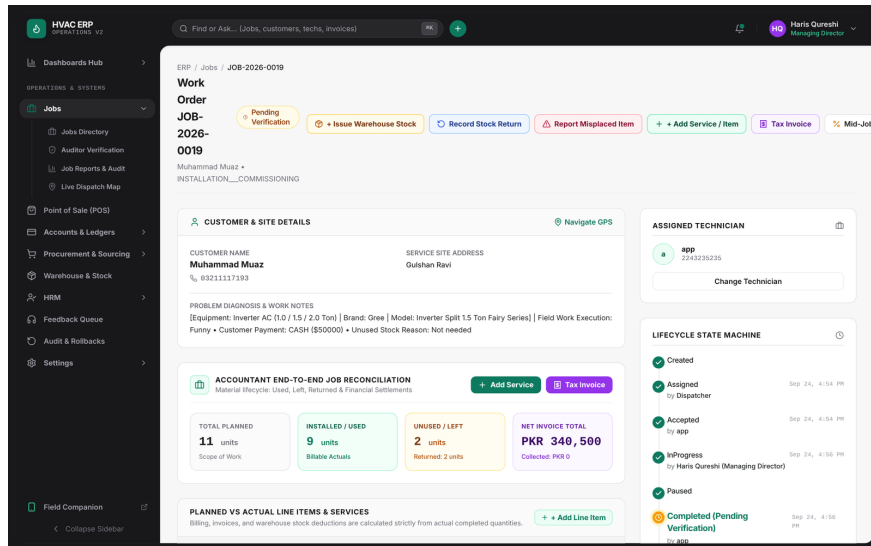
Job detail after complete — photos & status on web
