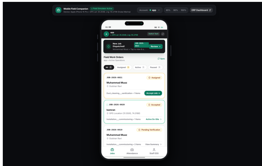
Mobile Field Companion — Jobs home (web simulator)
