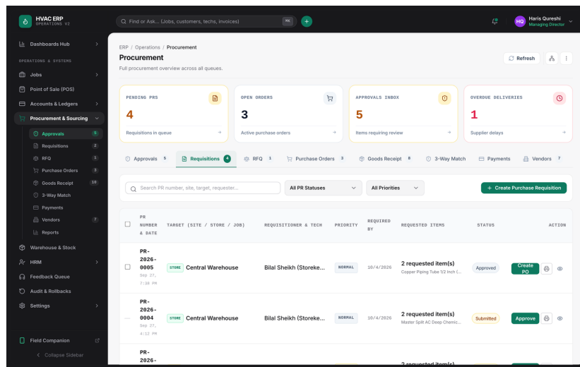
Procurement overview / Requisitions tab
