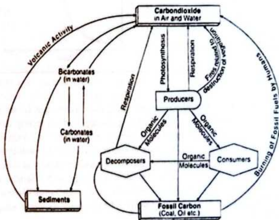
Figure.2: Carbon Cycle
