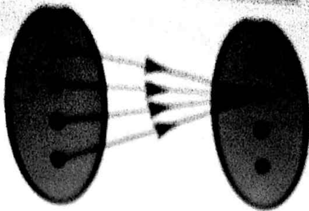
Figure 1 Constant Mapping
