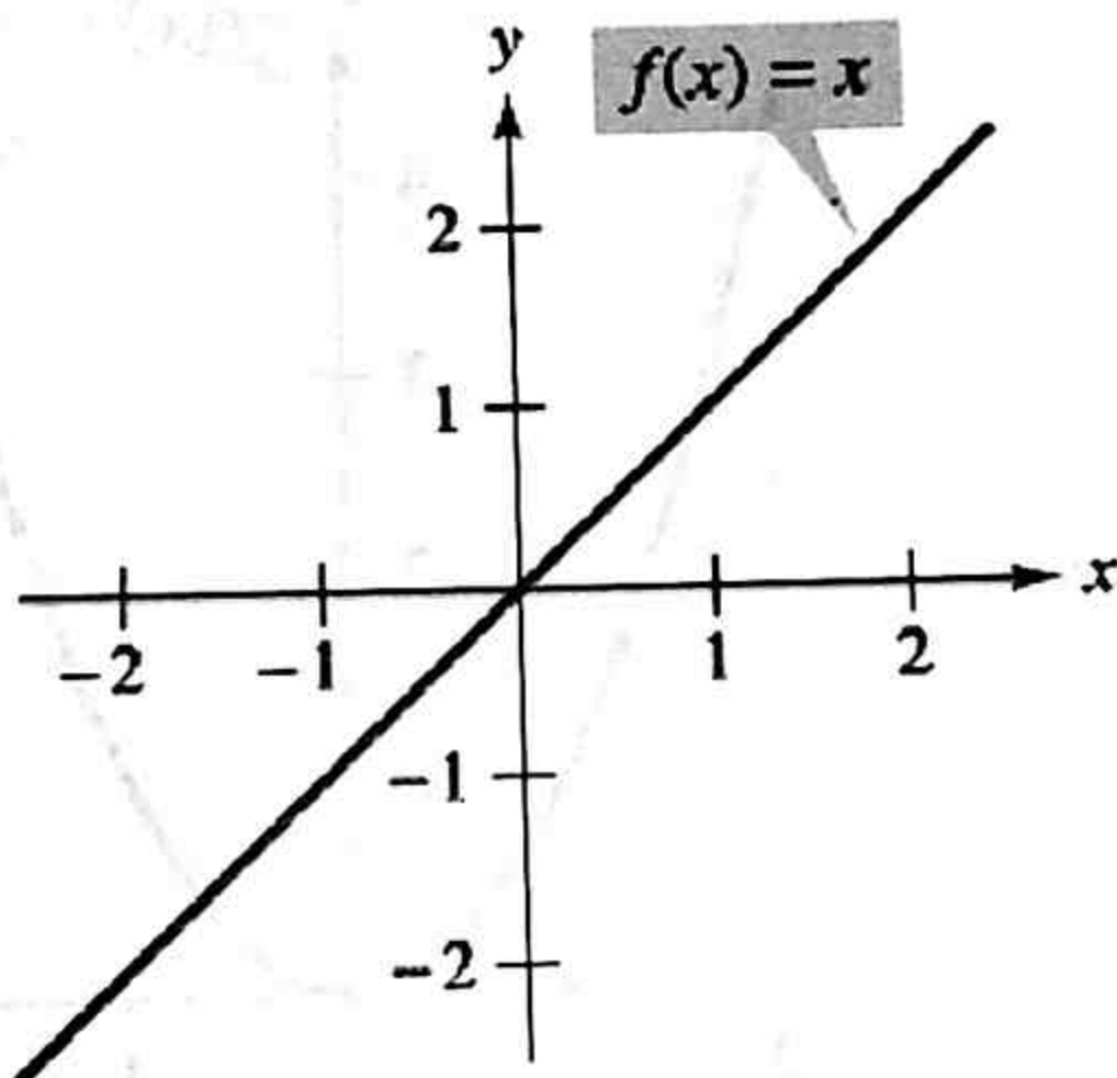
Figure 6: Identity Function
