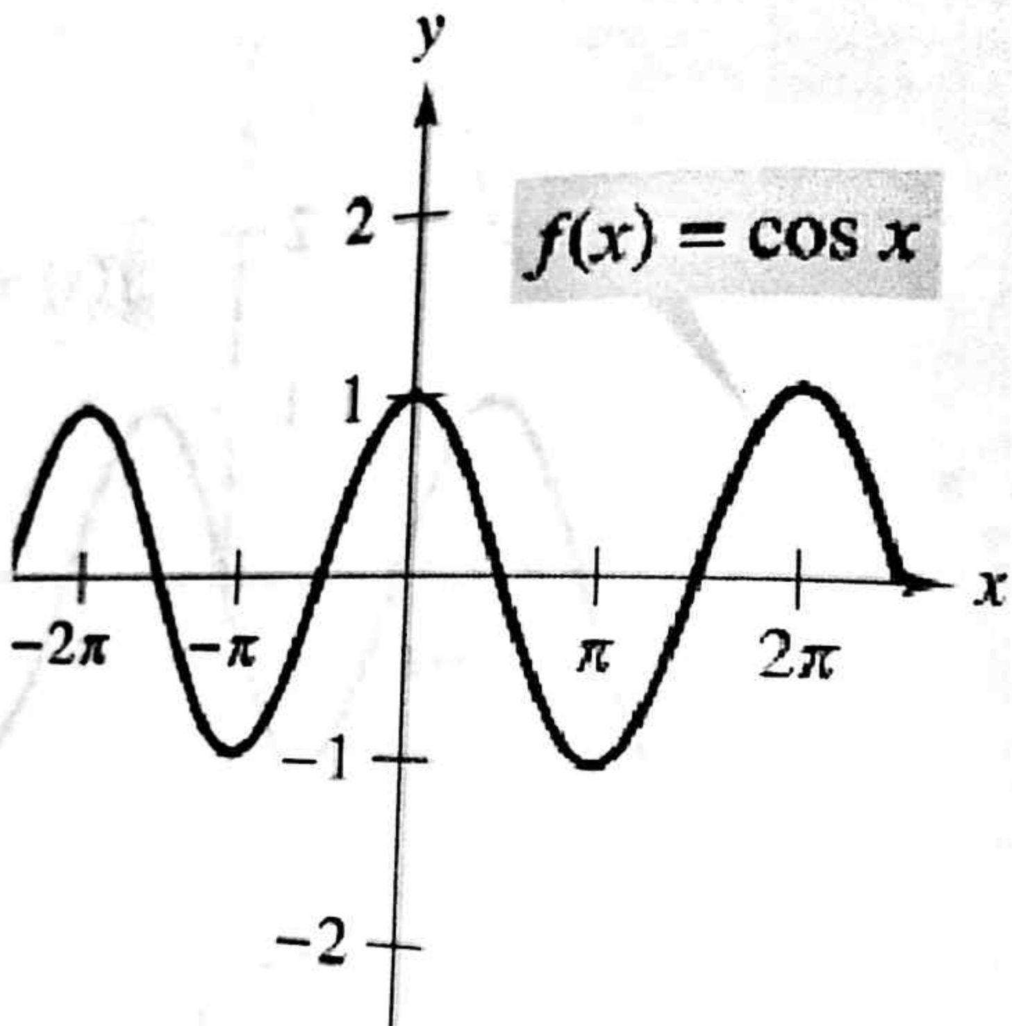
Figure 13: Cosine Function
