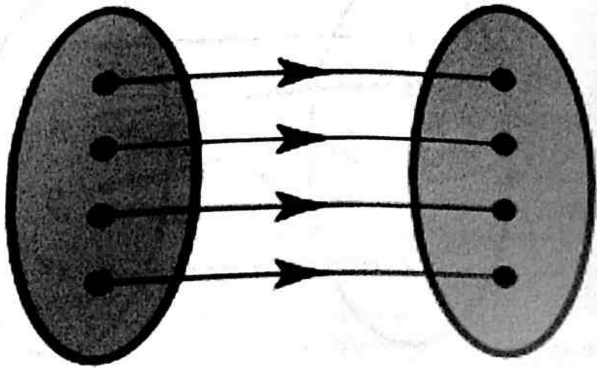
Figure 2: One-One Mapping
