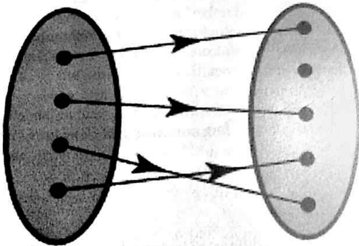
Figure 3: One-One Mapping
