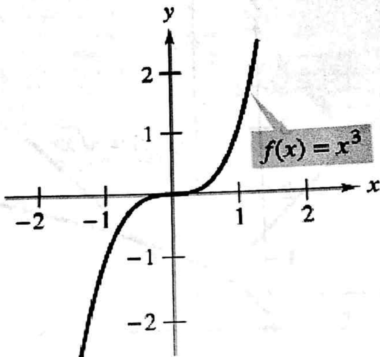
Figure 8: Cubing Function
