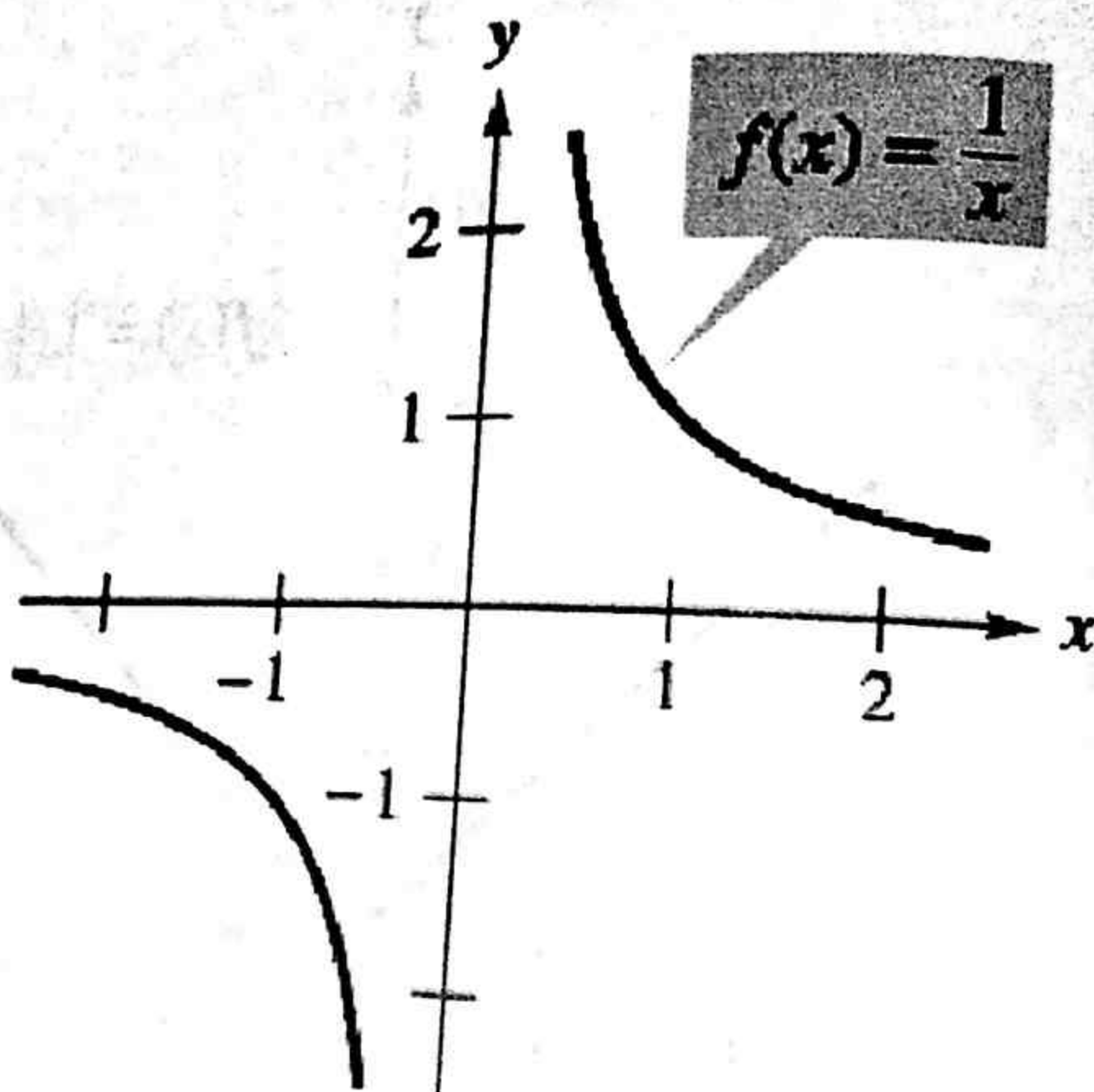
Figure 11: Rational Function
