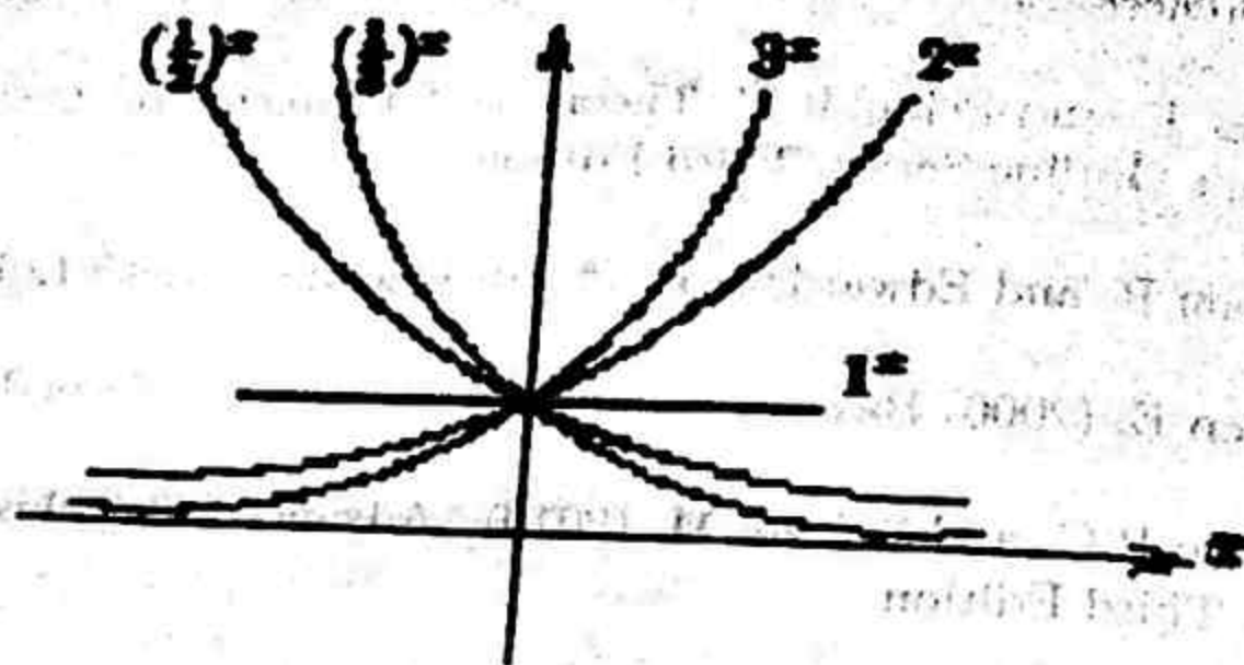
Figure 5: Exponential Function
