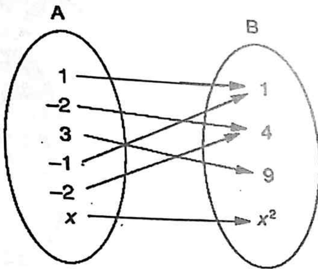
Figure 1: Mapping
