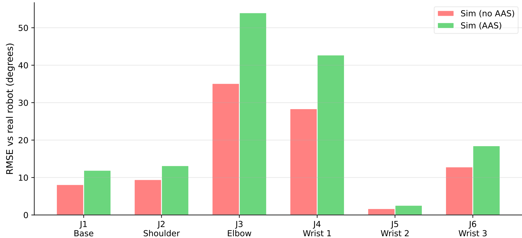
Joint position RMSE: simulation pipelines vs real robot
