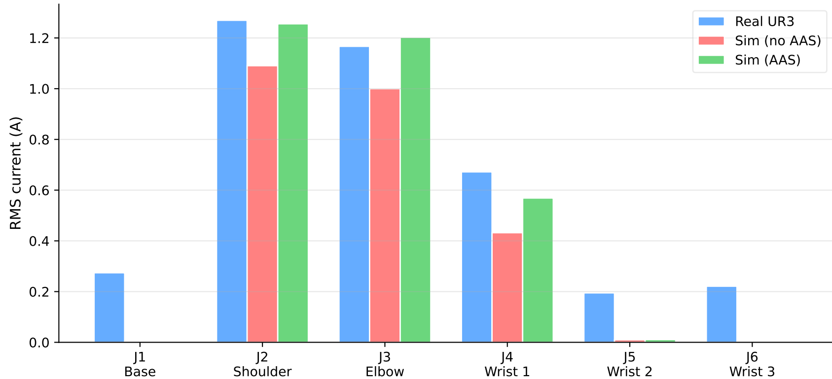
RMS joint current by pipeline
