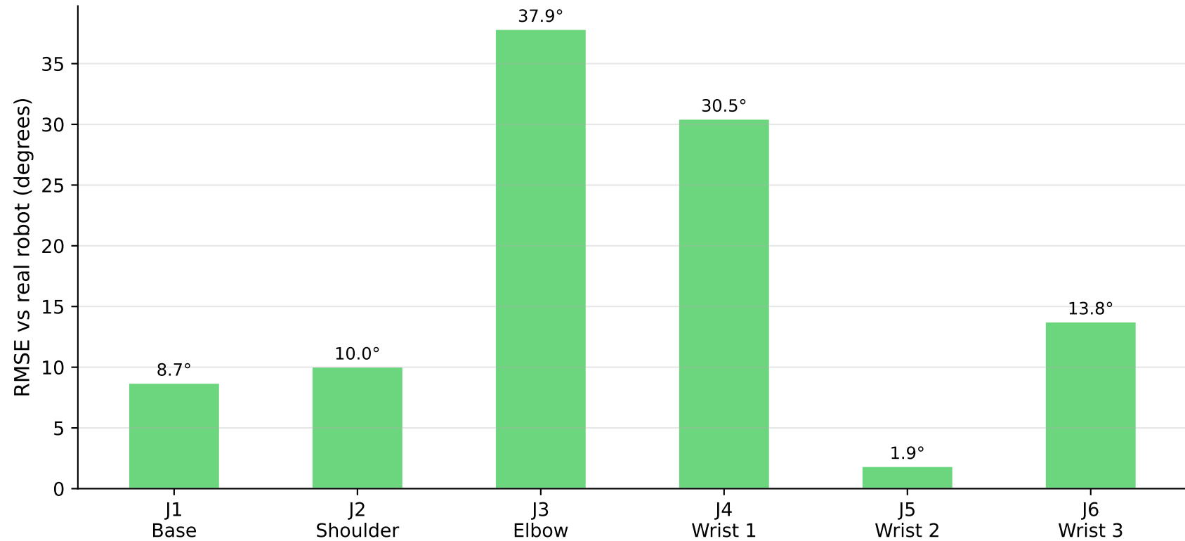
Joint position RMSE: Pipeline 2 vs Real robot
