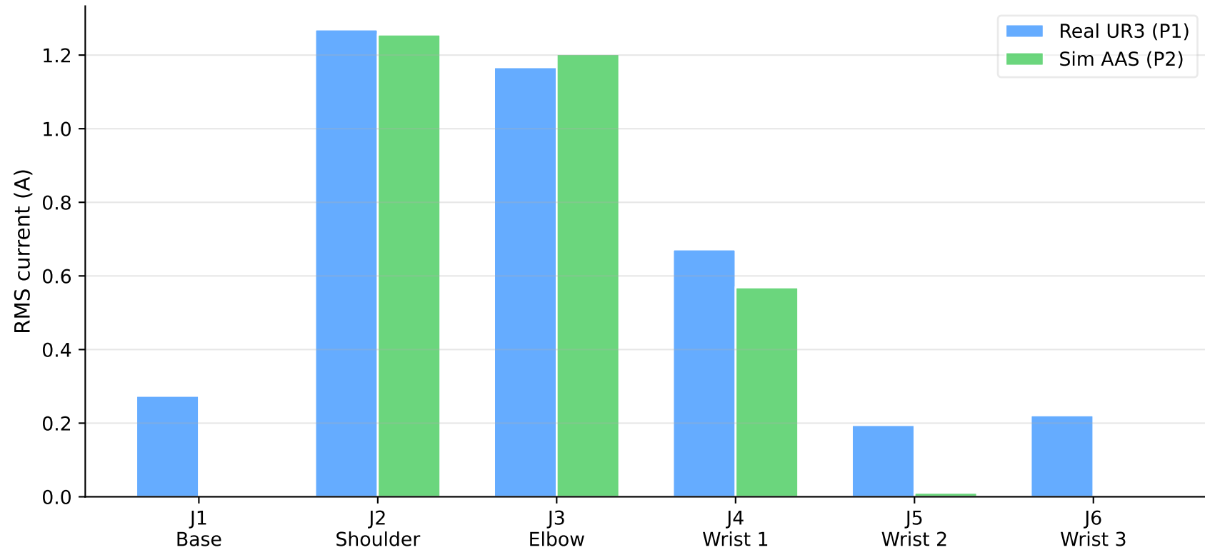
RMS joint current: Pipeline 2 vs Real robot
