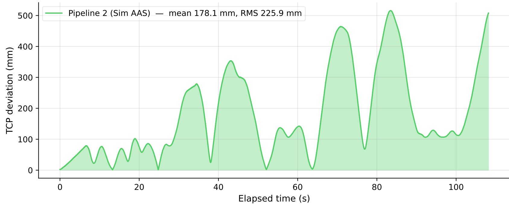
TCP path deviation: Pipeline 2 vs Real robot
