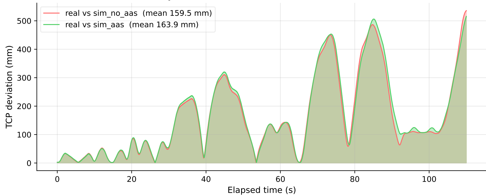
TCP path deviation from real robot over time
