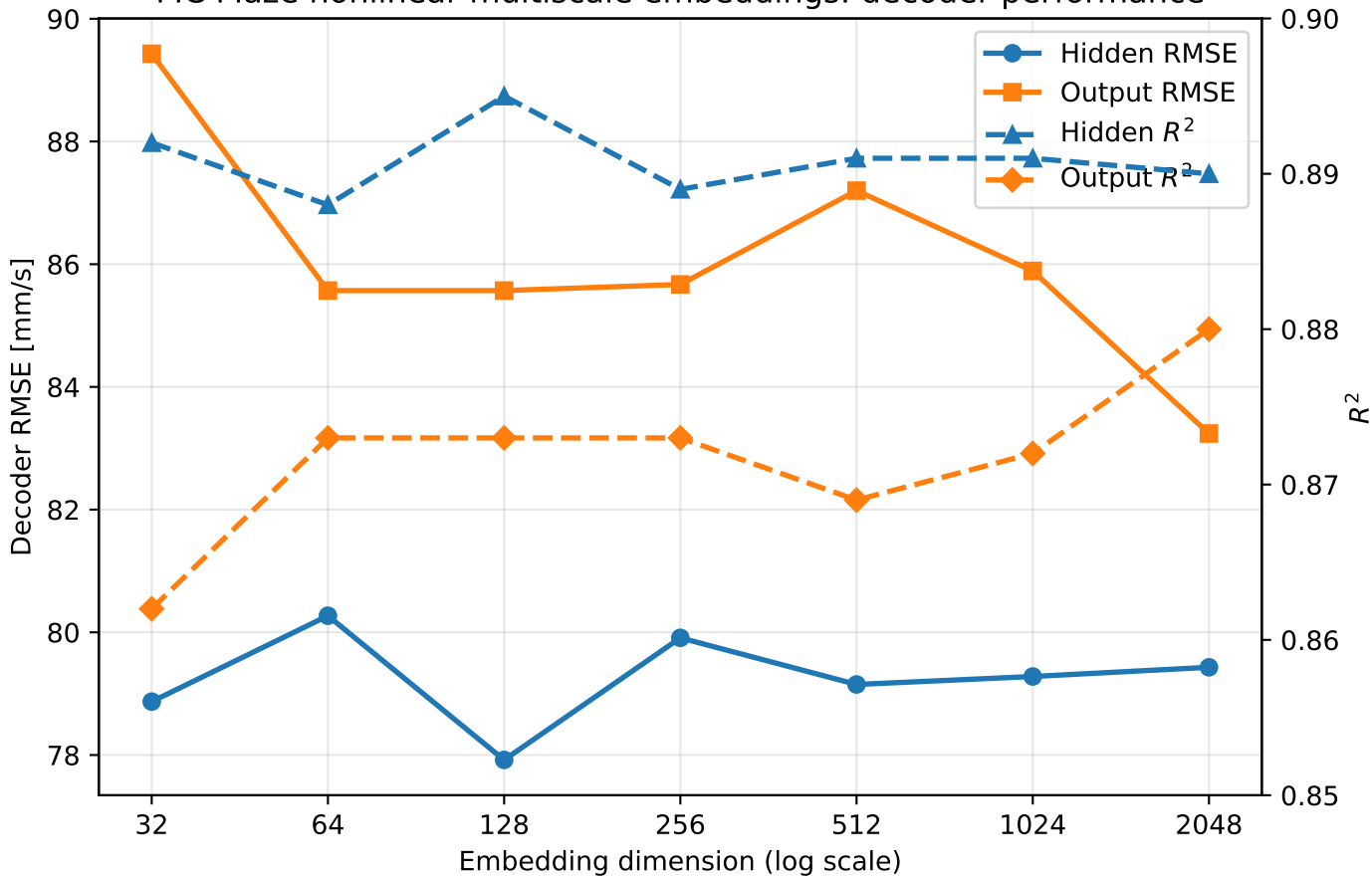
MC Maze nonlinear multiscale embeddings: decoder performance
