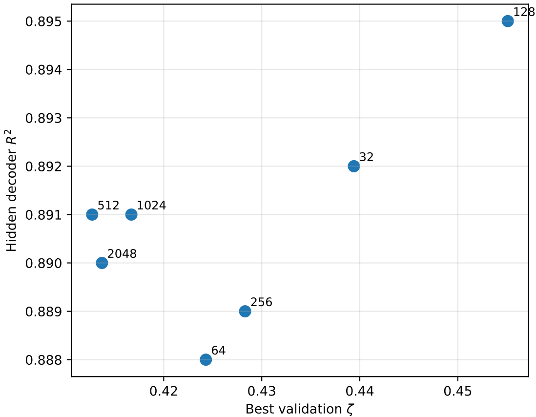
Hidden R^2 vs. validation \zeta
