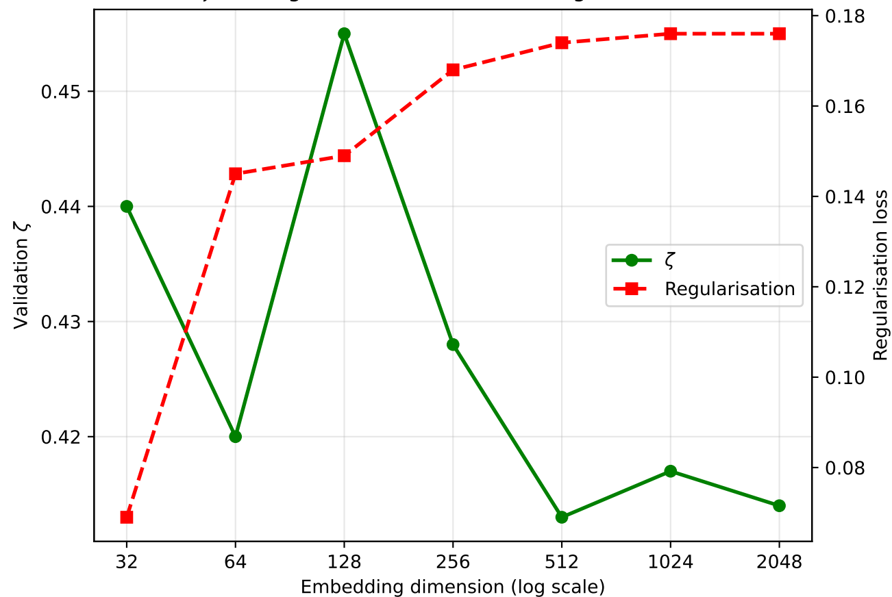
\zeta and regularisation vs. embedding dimension
