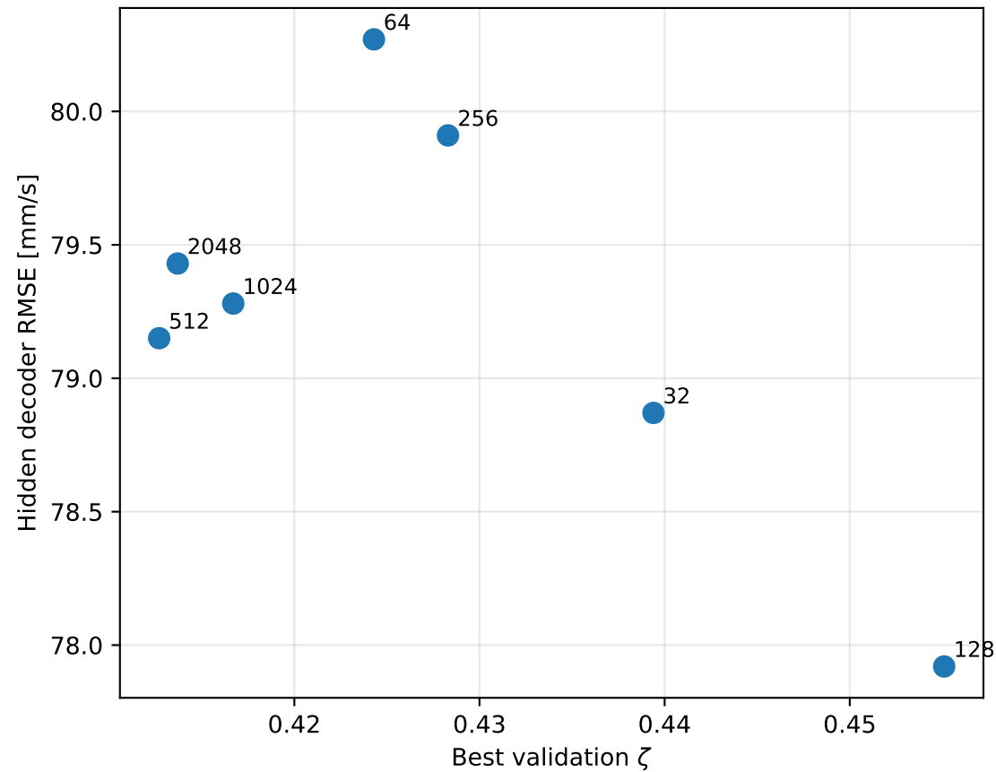
Hidden RMSE vs. validation \zeta
